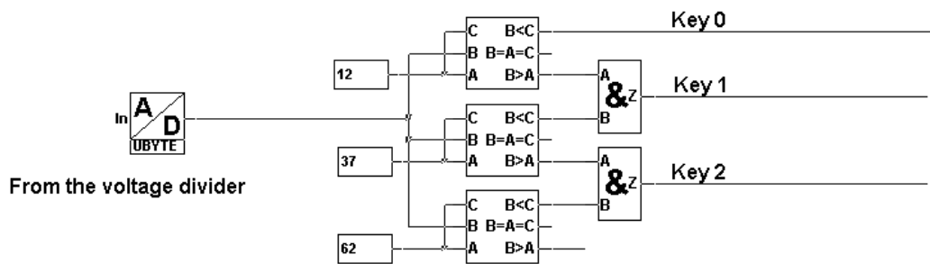
Figure B8 Key Recognition by Analog Value Evaluation
